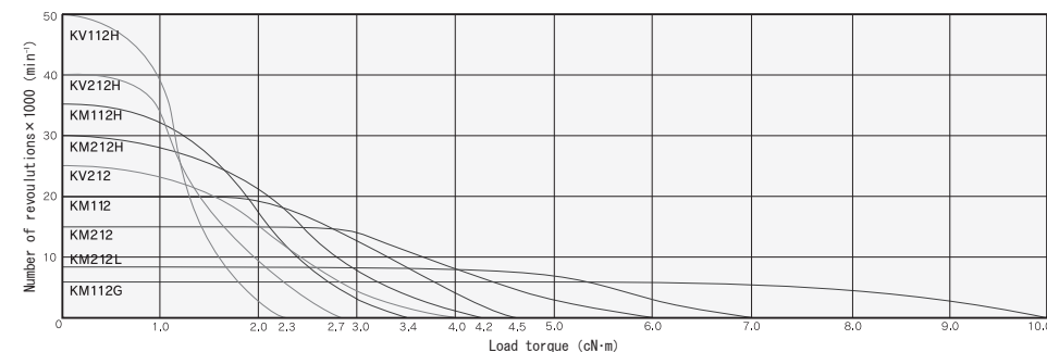
fig-4. Speed / Torque Curve
